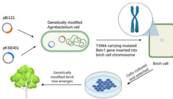
Figure 3. Transformation of birch cells via Agrobacterium to enable the acquisition of both a mutated Bet v 1 allele as well as a CRISPR-Cas9 mechanism in order to develop hypoallergenic trees.
