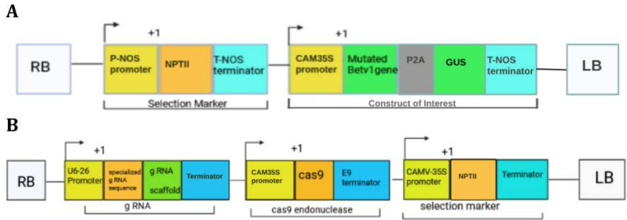
Figure 4. (A) pBI121: Genetic circuit for the expression of mutated Bet v 1 in birch cells, as well as an antibiotic resistance and GUS reporter gene. (B) pKSE401: Genetic circuit for the expression of a CRISPR-Cas9 construct, including a gene for the expression of a gRNA, a cas9 protein, and antibiotic resistance. Both systems are contained within left border (LB) and right border (RB) sequences, with transcription start sites marked as the +1 nucleotide. (A)'s genetic circuit has been modified from Lal et al., 2024; the mutated Bet v 1 allele was introduced, along with the P2A sequence and GUS reporter system, under the CaMV 35S promoter. (B)'s genetic circuit has been modified from an existing vector proposed by Xing et al., 2014.
