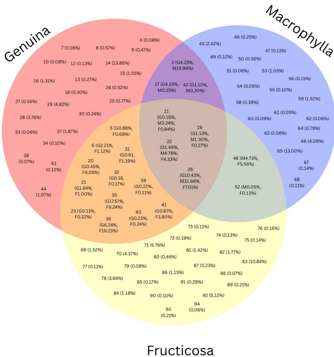
Figure 3. A Venn Diagram Showing the Distribution of VOCs in the Three C. odorata varieties
