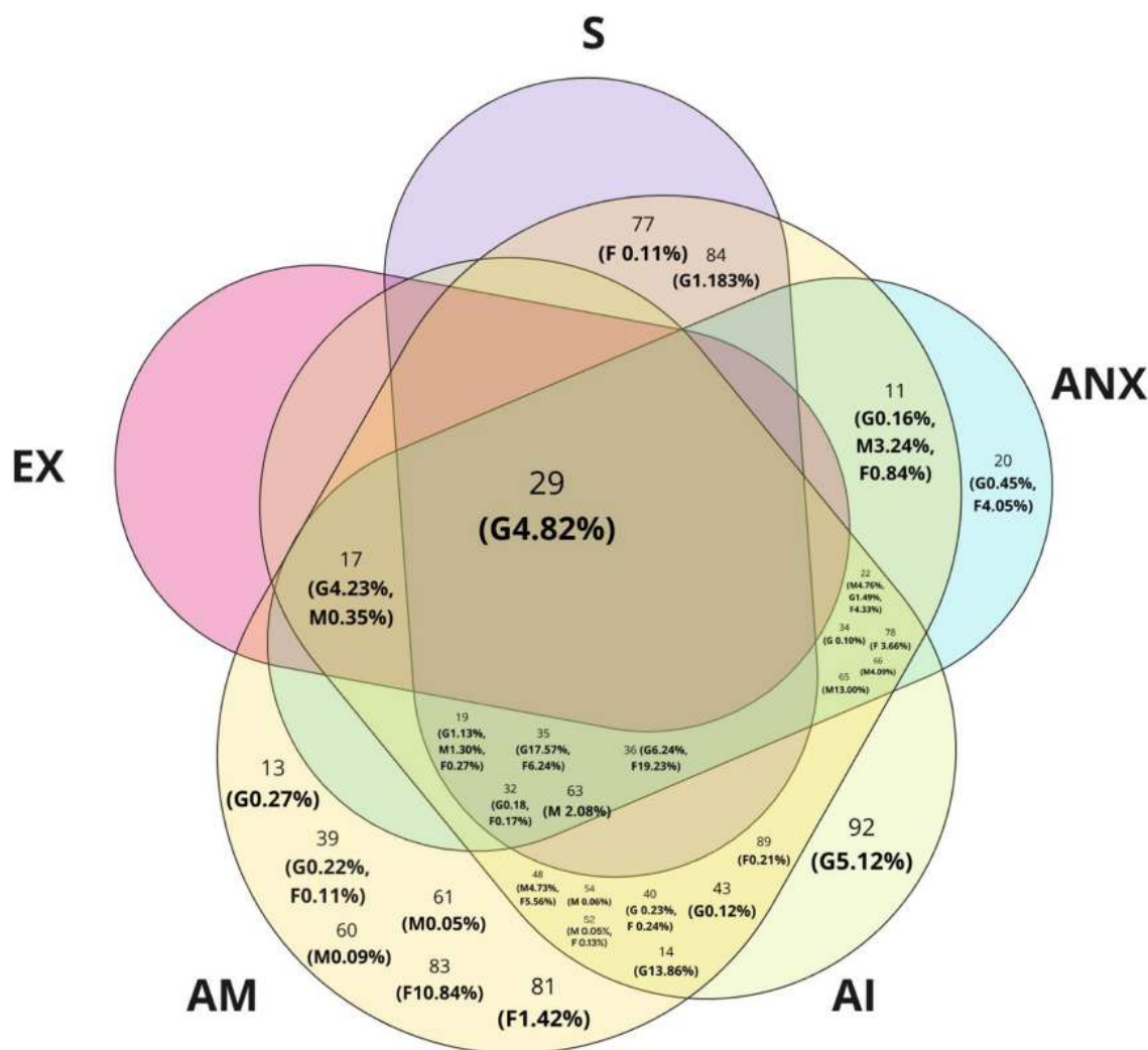
Figure 2. A Venn Diagram Illustrating the Distribution of VOCs in Five Therapeutic Categories
